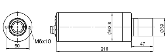
CT18 (unit: mm)
