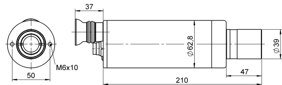
CT18 with viewfinder option (unit: mm)
